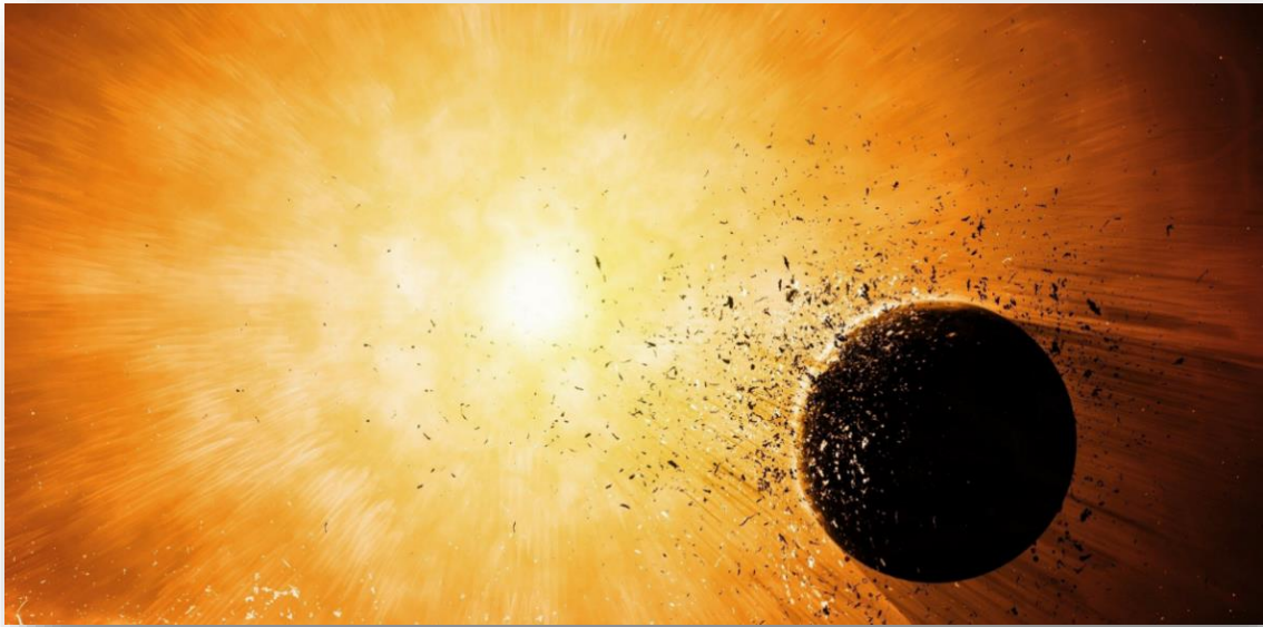
Fig. 29. Was the supernova explosion in the Orion Nebula 5 million years ago due to a space war where atomic weapons of mass destruction were used?
