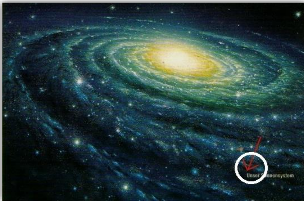
Fig.1. The Milky Way Galaxy and the part we are covering in these papers (with a few exceptions). The arrow points out our solar system, but the white circle covers pretty well the tiny bit of space we are mostly going to cover in this paper. Although it doesn't look like much, the circle covers many, many light-years.
