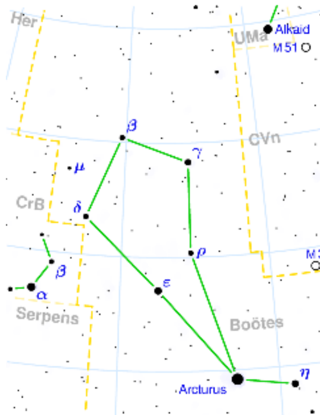
Fig. 26. Arcturus in the Boötes Constellation.
