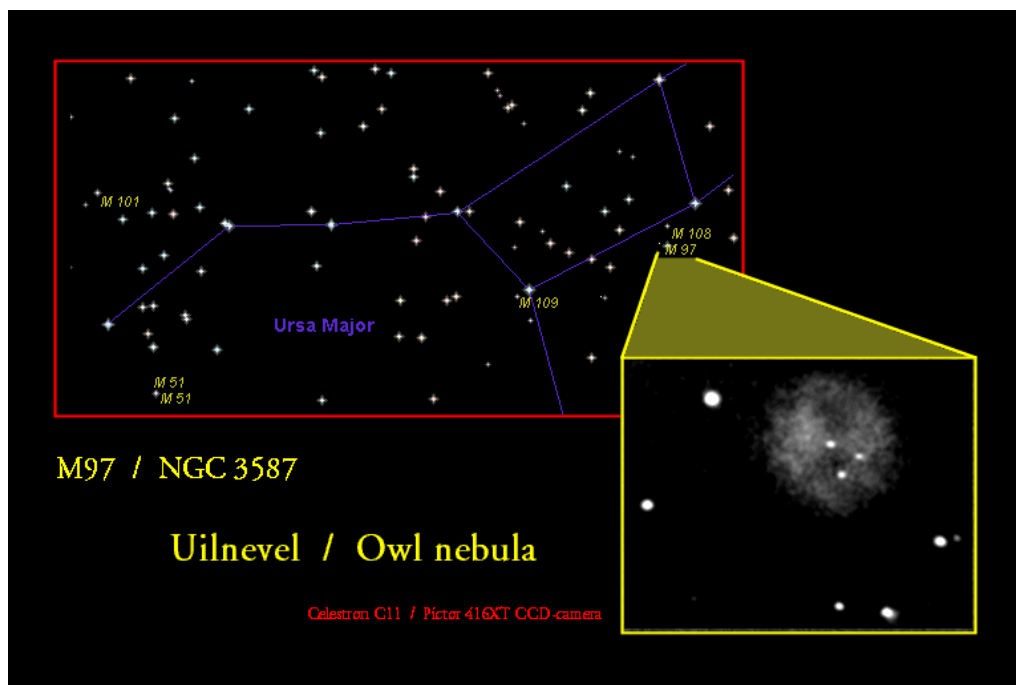
Fig. 9. “Messier 97” (M97) or “New General Catalogue 3587” (NGC 3587) 12 The Owl Nebula.
